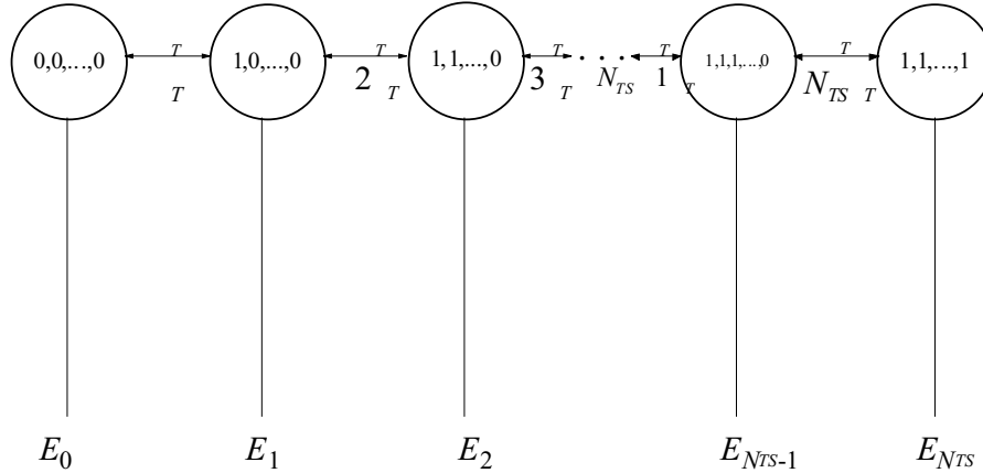
Figure 5. Markov chain model for TDMA system with ordered hunt and reallocation of the slots
