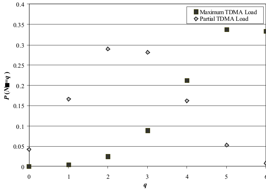
Figure 2. Probability density function of N_T for a_T=48.7Erl and a_T=25Erl , considering a normal slots allocation and W_C=1.2288MHz
