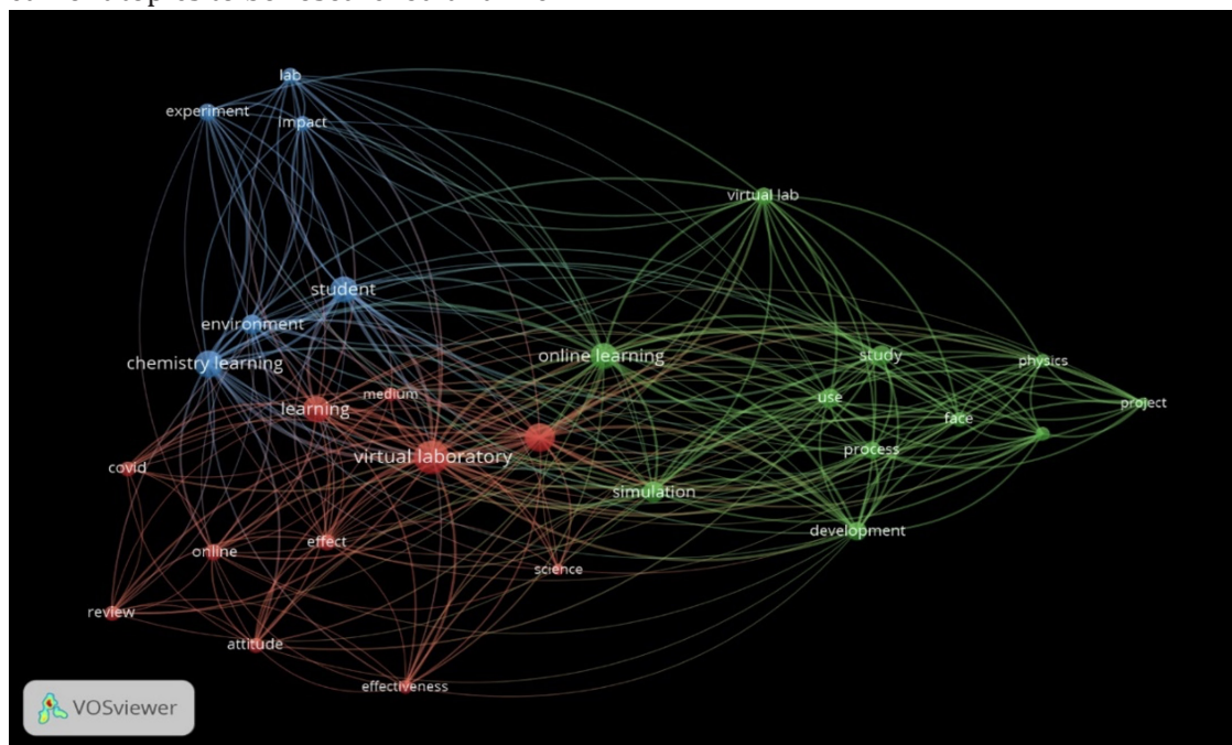
FIGURE 2. Network Visualization.
