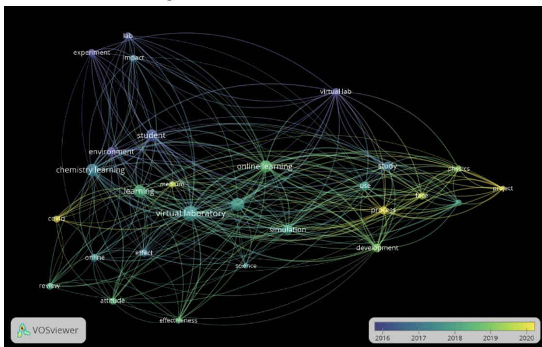
FIGURE 3. Overlay Visualization.
