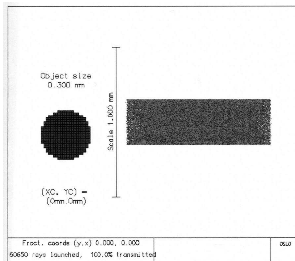
Fig. 7. Ray trace of the system for a round entrance image that produces the illuminated strip on the back side of the plate.
