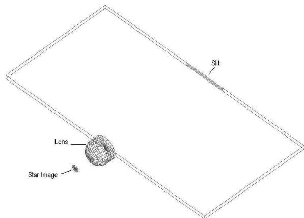
Fig. 4. Design of the shape transformer showing the star image from the telescope, the magnifying lens, the plate, and the exit slit.
