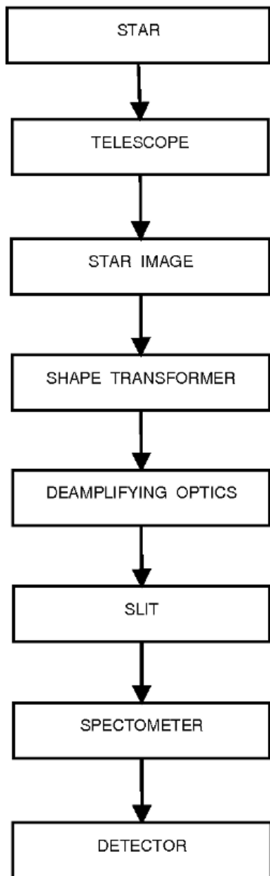
Fig. 1. The flow of light from the star to the detector, passing through the shape transformer.
