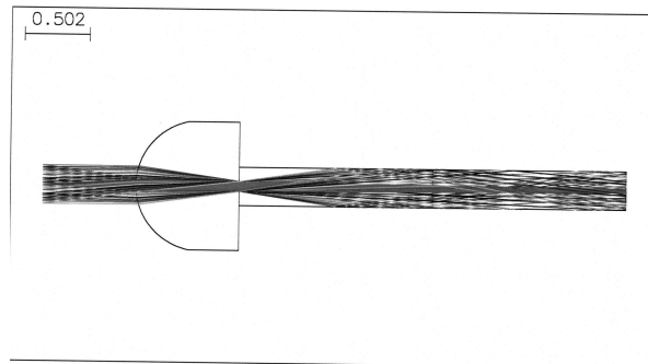
Fig. 5. Meridional ray trace of the transformer showing the waist of the beam and the internal reflections.
