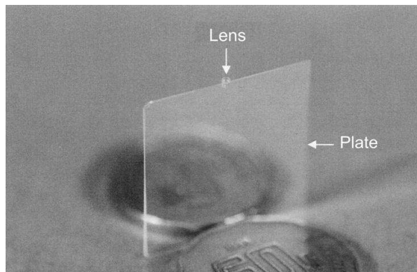
Fig. 6. Star shape transformer in the laboratory, composed of a one-millimeter diameter lens and a glass plate.
