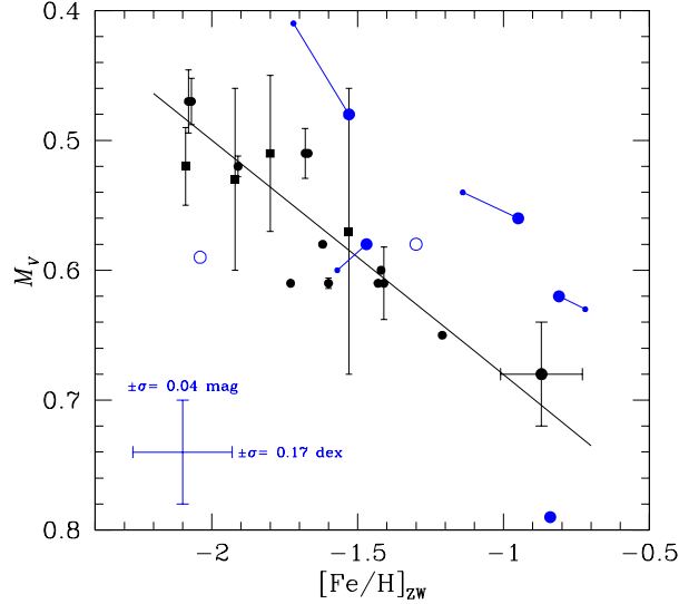
Fig. 4. M_v - [\text{Fe}/\text{H}] relation derived from cluster RR Lyrae stars (Arellano Ferro et al. 2008a). Blue points are the five RRAb stars in our sample. When available, two positions are given; the larger points are the finally adopted solution while the smaller points correspond to similar solutions with smaller number of harmonics. Open blue circles correspond to the two RRC stars in our sample. The uncertainties in the values of the blue symbols are discussed in the text and indicated by the blue error bars. See electronic version for the color coding.
