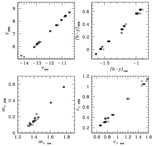
Fig. 1. Transformations from the instrumental to the standard uvby system for the magnitude and colors. See equations (1–5).
