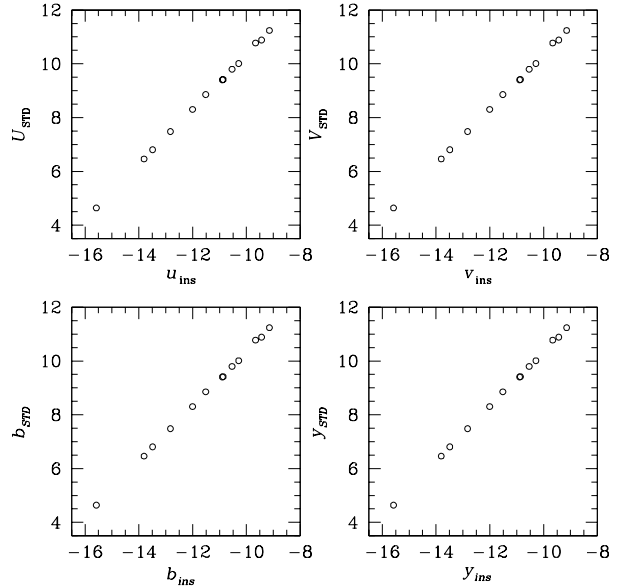
Fig. 2. Transformations from the instrumental uvby magnitudes to the standard system. See equations (6–9).
