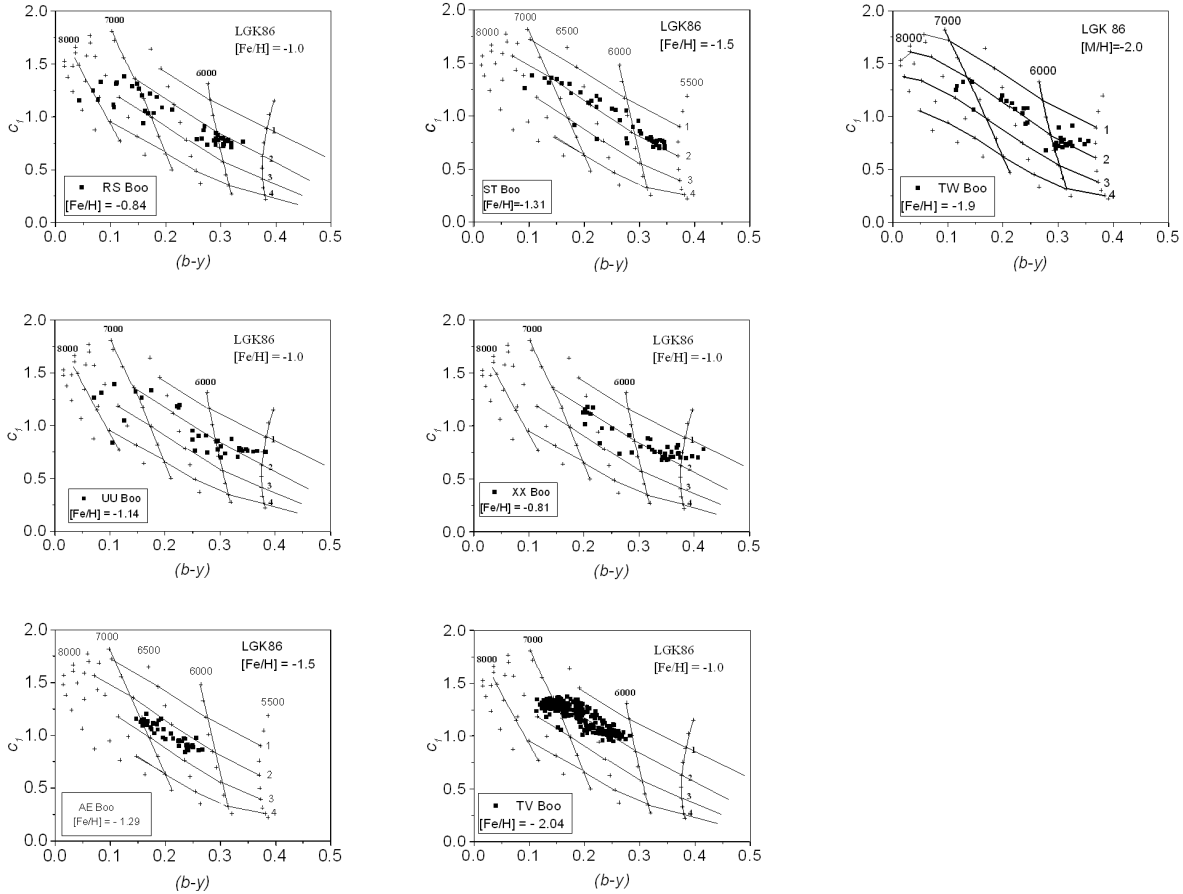
Fig. 5. Model grids on the (b - y)_0 - c_0 plane along the stellar variations through the cycle.
